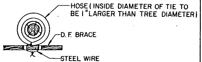
TIE DETAIL
