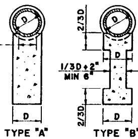
WALL SECTION
